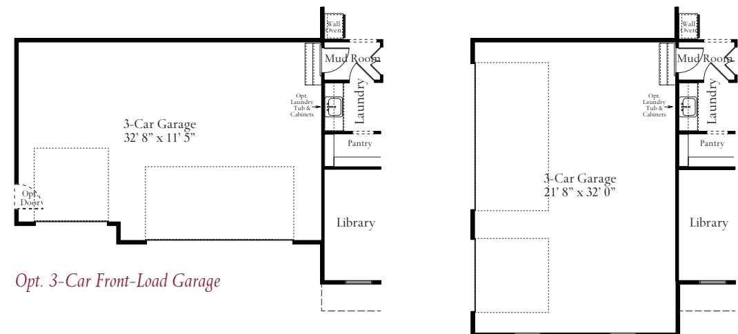
Opt. 3-Car Side-Load Garage
