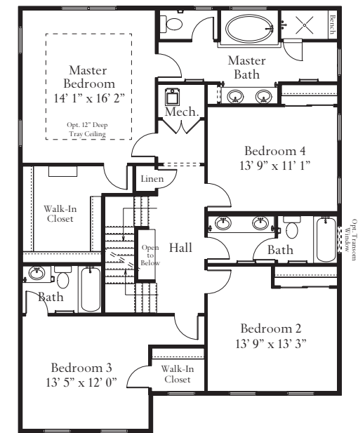
Alternate Second Floor with Opt. Third Bath and Opt. Master Bathroom
